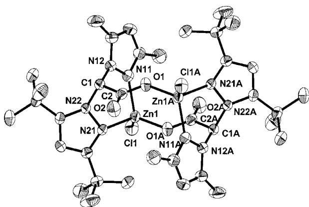
Figure 3. Molecular structure of [\text{Zn}(\text{bpa}^{\text{tBu}_2, \text{Me}_2})\text{Cl}]_2 ( 5 ); thermal ellipsoids are drawn at the 50% probability level
