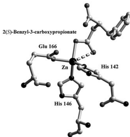
Figure 1. Active site of thermolysin with inhibitor (2 S )-2-benzyl-3-carboxypropionic acid bound to a zinc ion (PDB-Code: 1HYT) [5]
