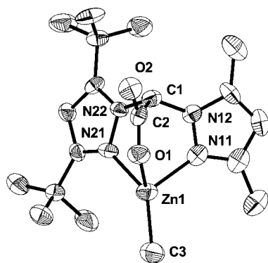
Figure 4. Molecular structure of [\text{Zn}(\text{bpa}^{\text{tBu2,Me2}})(\text{CH}_3)] ( 8 ); thermal ellipsoids are drawn at the 50% probability level
