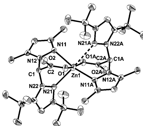
Figure 5. Molecular structure of [\text{Zn}(\text{bpa}^{\text{tBu2,Me2}})_2] ( 11 ); thermal ellipsoids are drawn at the 50% probability level; only one of the zinc positions is shown
