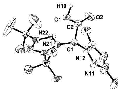
Figure 2. Molecular structure of bpaH tBu2,Me2 ( 4 ); thermal ellipsoids are drawn at the 50% probability level
